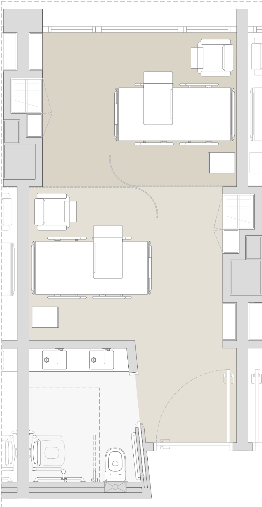
PLANTA e=1/40
